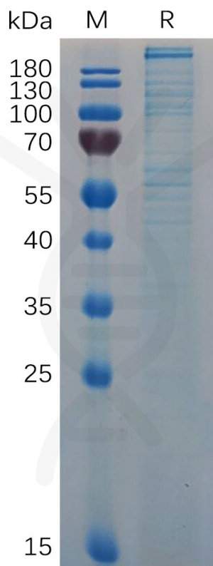
Figure 1. Mouse VWF (23-2813) Protein, His Tag on SDS-PAGE under reducing condition.
