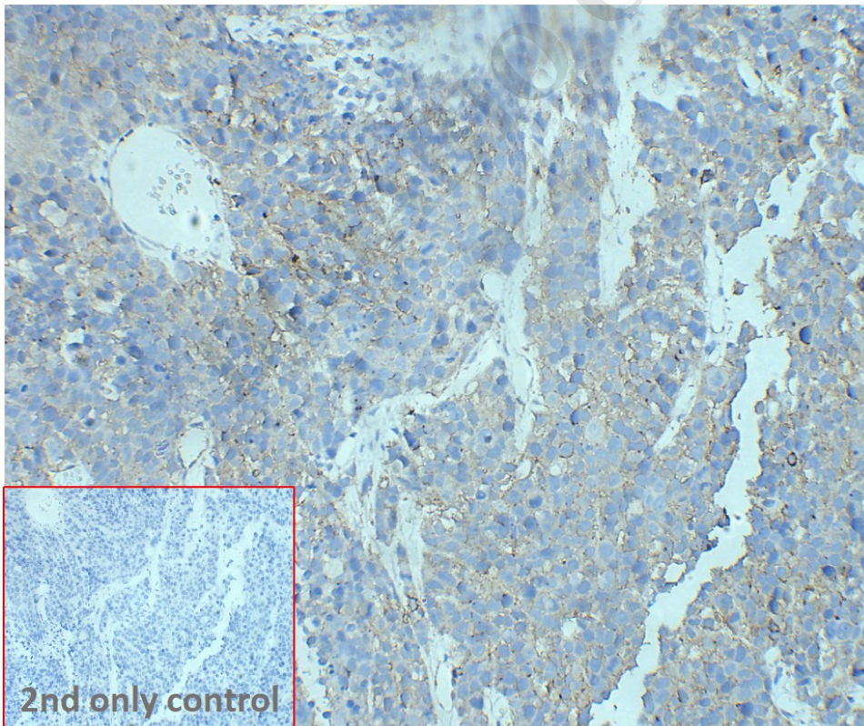
Figure 1. IHC analysis of M-NSG LnCap DiSliceX™ SlideSet section (Cat. No. SLI100015) with Anti-CD99 antibody (DM203) Rabbit mAb (Cat. No. DME100203) at a concentration of 10 μg/ml. The inset image shows the absence of staining in secondary antibody-only control.
