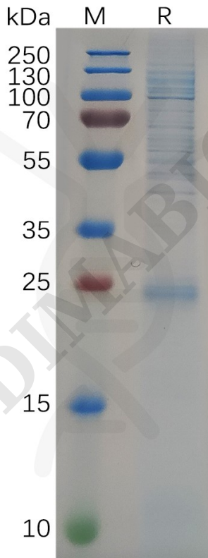
Figure 1. Human KRAS Protein, His Tag on SDS-PAGE under reducing condition.
