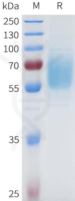
Figure 1. Human EGFR(301-645) Protein, His Tag on SDS-PAGE under reducing condition.
