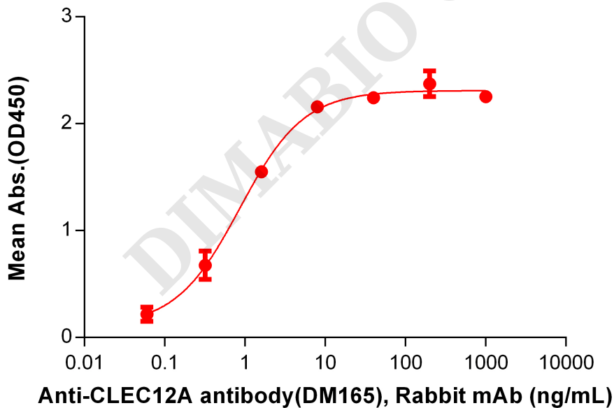
Figure 2. ELISA plate pre-coated by 2 \mu g/mL (100 \mu L/well) Human CLEC12A Protein, His Tag (PME100096) can bind Anti-CLEC12A antibody(DM165), Rabbit mAb in a linear range of 0.32-1.60 ng/mL.
