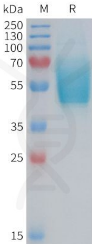
Figure 1. Human CGRPR Protein, mFc Tag on SDS-PAGE under reducing condition.
