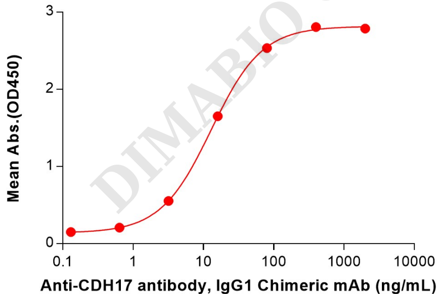
Figure 2. ELISA plate pre-coated by 2 \mu\text{g}/\text{mL} (100 \mu\text{L}/\text{well} ) Human CDH17(450-566) Protein, hFc Tag (PME101566) can bind Anti-CDH17 antibody, IgG1 Chimeric mAb in a linear range of 3.20-80 ng/mL.
