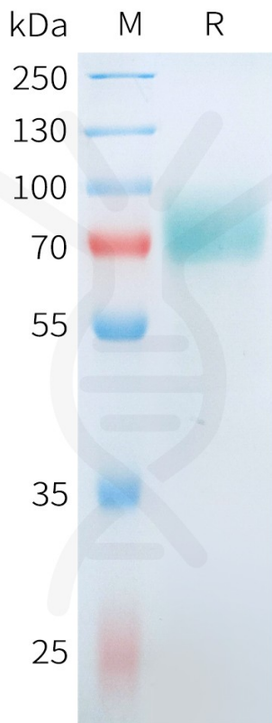
Figure 1. Human CD19(M75V,R76S,F85S) Protein, hFc Tag on SDS-PAGE under reducing condition.
