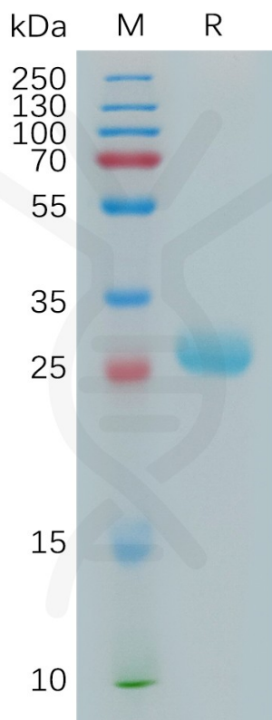
Figure 1. Human BTN3A2 Protein, His Tag on SDS-PAGE under reducing condition.
