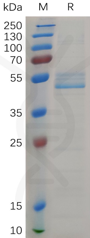
Figure 1. Cynomolgus MDK Protein, hFc Tag on SDS-PAGE under reducing condition.
