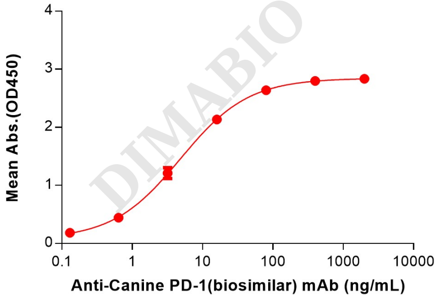
Figure 2. ELISA plate pre-coated by 2 \mu\text{g}/\text{mL} (100 \mu\text{L}/\text{well} ) Canine PD-1 Protein, hFc Tag (PME-D100008) can bind Anti-Canine PD-1 (INTERVET 4F12) mAb (BME100202) in a linear range of 0.64–80 ng/mL.
