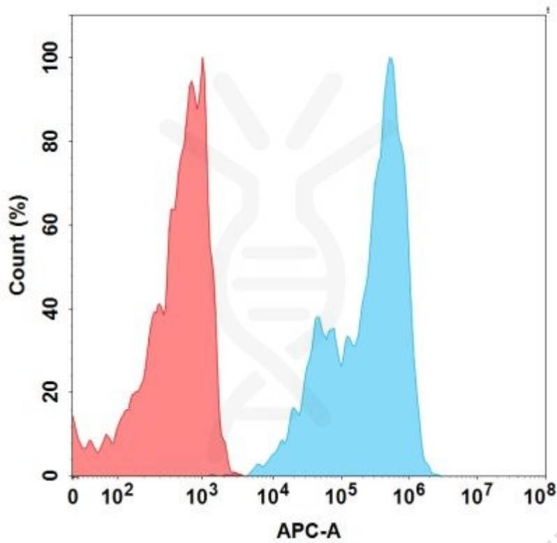
Figure 1. Flow cytometry analysis with 1 \mu\text{g}/\text{mL} Anti-IL7RA (lusvertikimab biosimilar) mAb (BME100084) on Expi293 cells transfected with Human IL7RA protein (Blue histogram) or Expi293 transfected with irrelevant protein (Red histogram).
